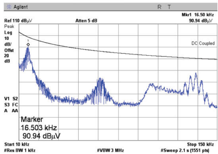
CE102 test results in 10-150 kHz range
