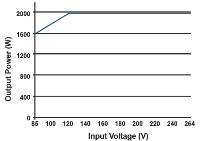
Line Derating Curve T4G-02D0 Model
