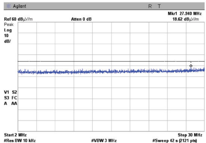
Radiated emission measurements results, in 2-30 MHz range
