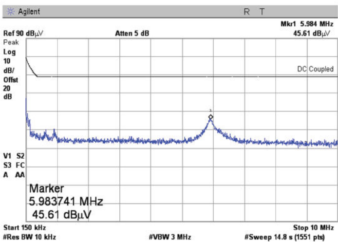
CE102 test results in 0.15-10 MHz range
